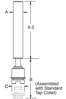
Straight Shank
